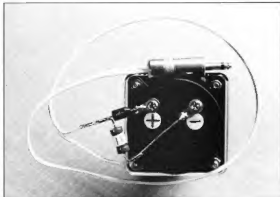
Figure III: The back of the milliammeter
